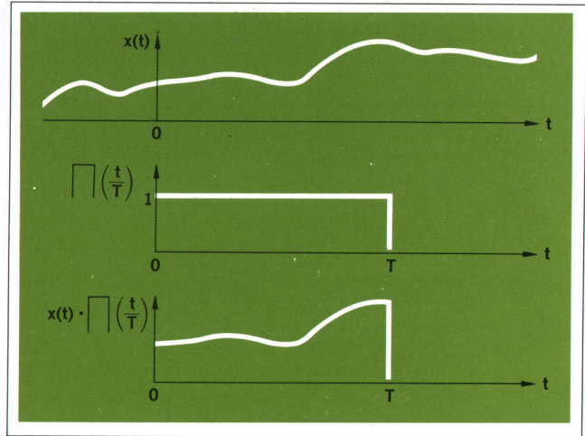
Fig. 6. When a T -second record is taken of an analog input, the effect is to multiply the input by a square window function. If the input isn't periodic with period T , the spectral lines of the input will not be lines but will have the \sin x/x shape shown in Fig. 7. To reduce this effect, Model 5450A Fourier Analyzer has built-in Hanning window-shaping functions.
