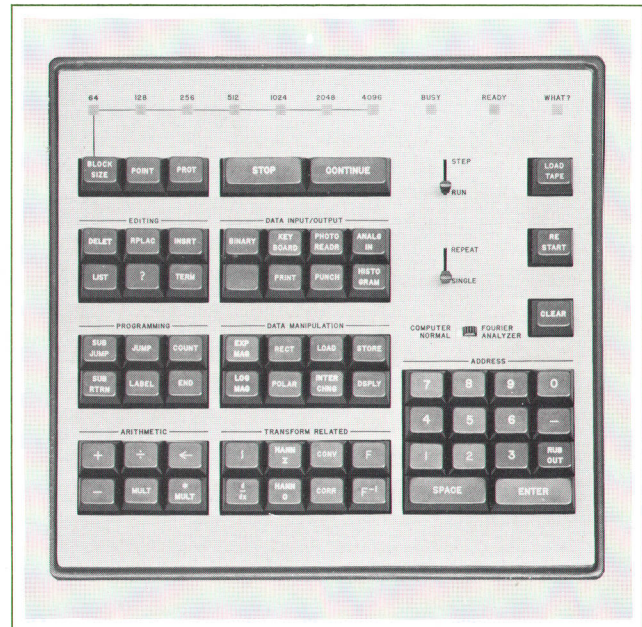
Fig. 2. All Fourier analyzer operations are keyboard controlled. The principal operations—Fourier transforms, convolution, correlation, complex multiplication, coordinate transformations, and so on—can be called for by single keystrokes, or strung together using the programming and editing features to form routines to be run automatically later on. Typical routines can change the analyzer into a spectrum analyzer, a correlator, an averager, and many other instruments.
