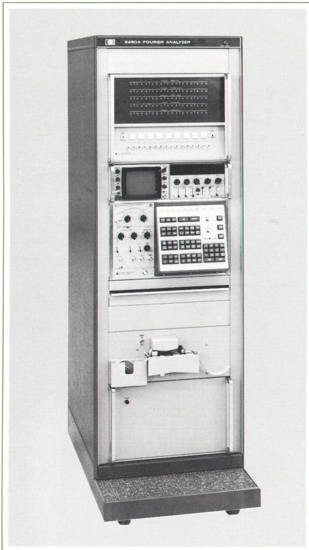
Fig. 1. Model 5450A Fourier Analyzer is a flexible, push-button-controlled, modular, digital instrument, useful for analyzing waveforms and time series in a wide variety of systems and processes. It uses a standard HP computer for memory and computation, but requires no knowledge of computer programming. When it isn't doing Fourier analysis, the computer can be used separately.
